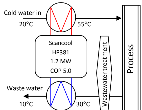
Basic concept for heat pump connection.
